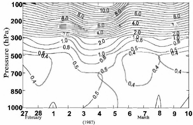
Fig. 5. Time height cross section of the area average potential vorticity values for the period 27 Feb. to 10 Mar. 1987
