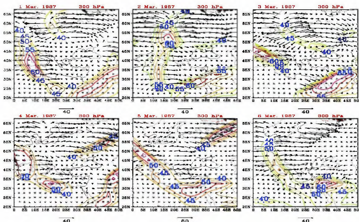
Fig. 10. Vector representation of the Q -vector field in the vicinity of the jet streams at 300 hPa for the selected period, overlapped with the contours of the jet streams greater than 40 m/s.
