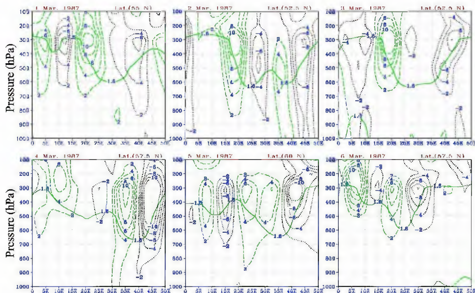
Fig. 11. Vertical cross section of Q (positive values dashed, negative values dotted) and the contour of the dynamical tropopause (solid).
